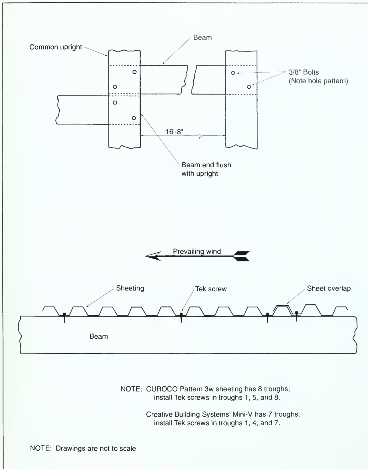
Figure 4. Apron and sheeting details.
